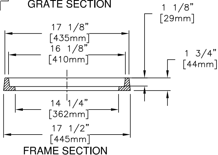
GRATE SECTION
